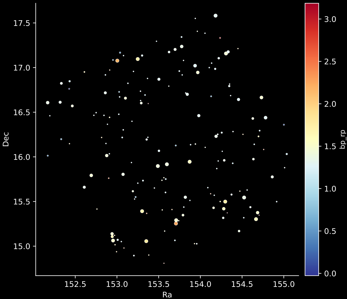
APOGEE DR17 Field: [K2_C4_170-31_btx] Stars: 172
