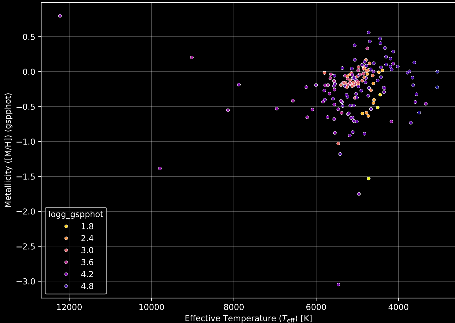
APOGEE DR17 Field: [K2_C4_170-31_btx] Stellar Population Parameters (n= 172)
