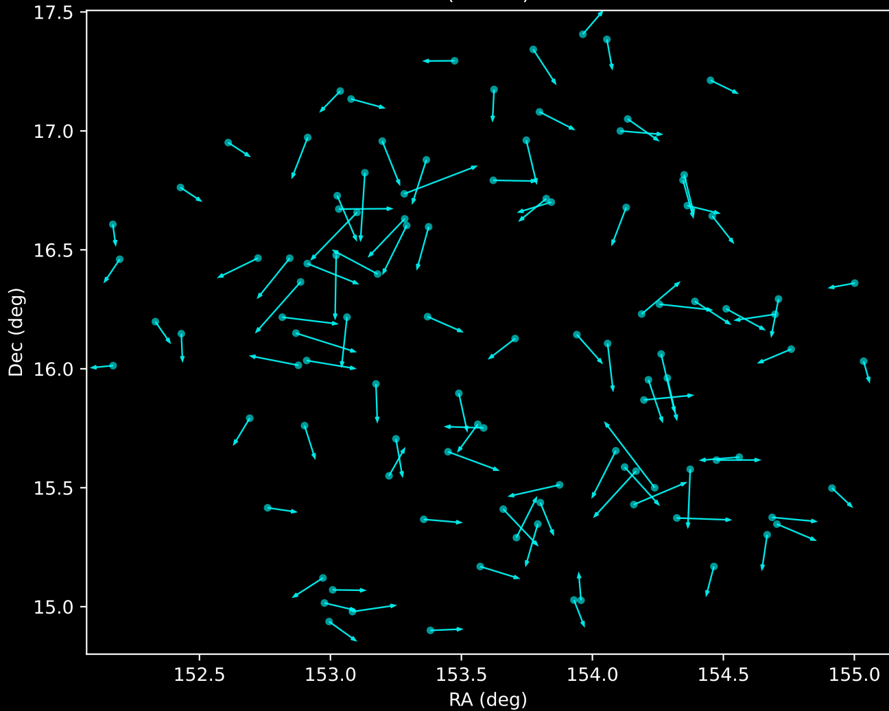
APOGEE DR17 Noise Stream Proper Motion Vectors (n=105)
