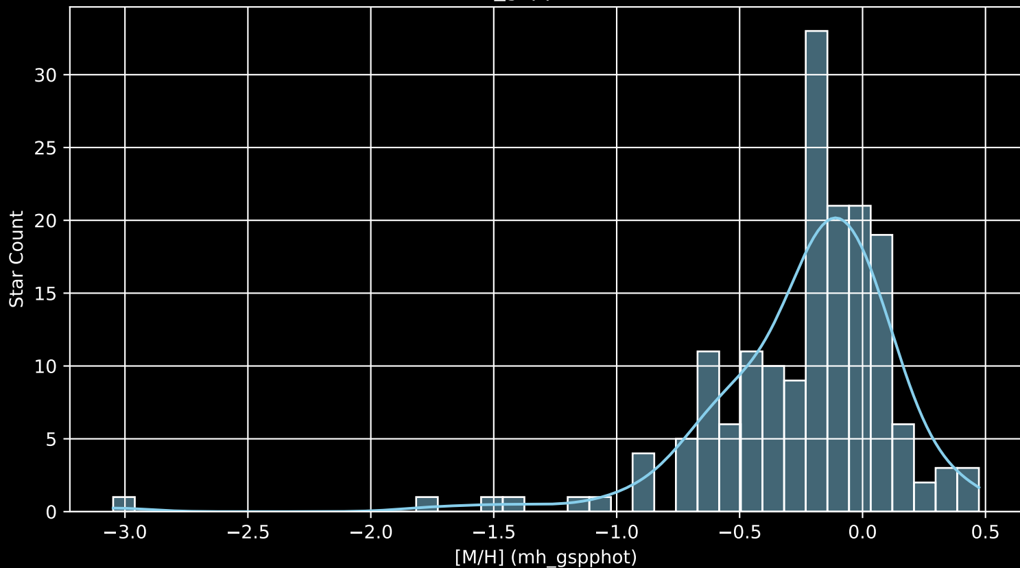
APOGEE DR17 Field: [K2_C4_170-31_btx [M/H] (mh_gspphot) (n= 170)
