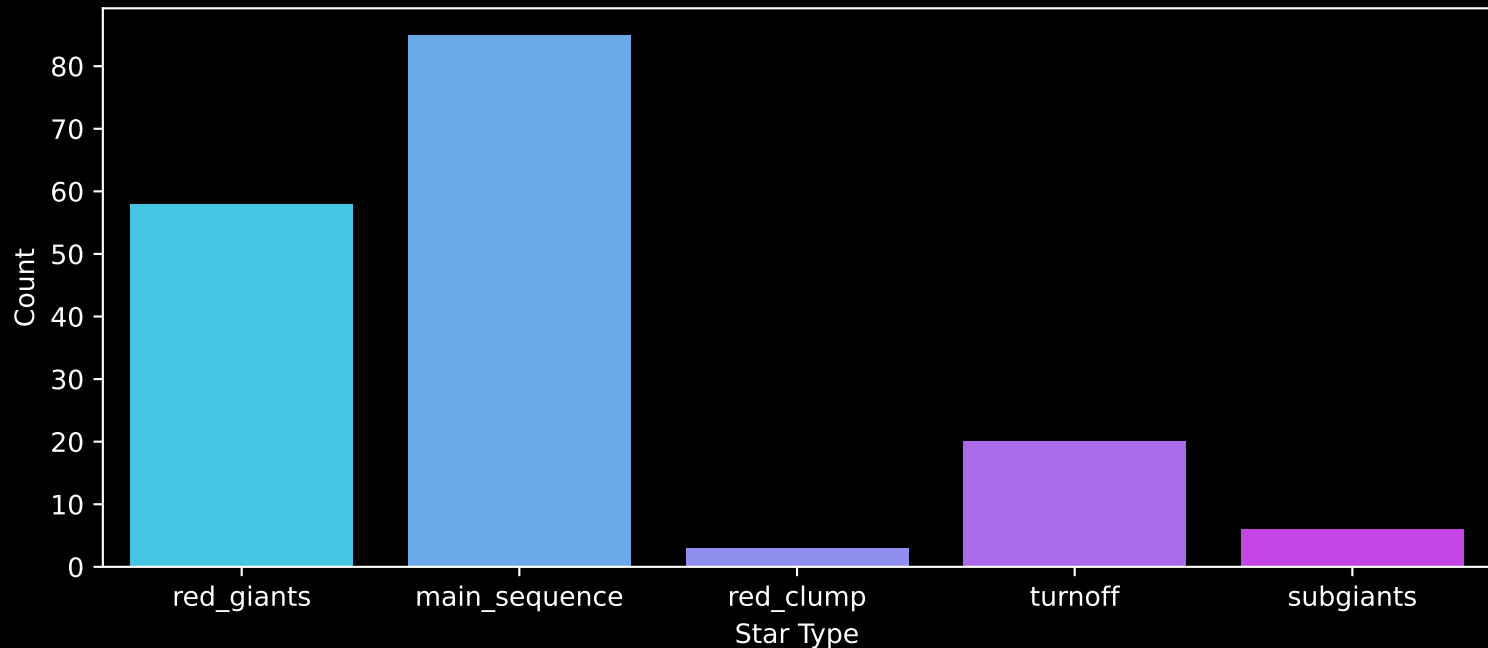
APOGEE DR17 Field: [K2_C4_170-31_btx] Count plot of Star Type
