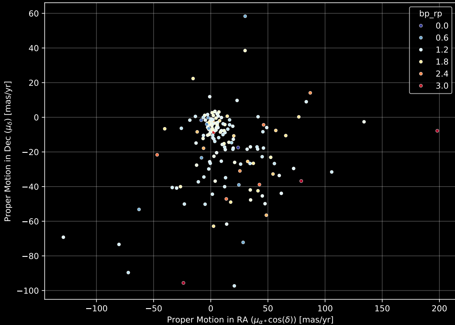
APOGEE DR17 Field: [K2_C4_170-31_btx] Proper Motion Diagram (n= 172)
