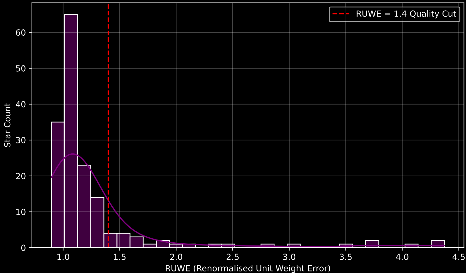
GAPOGEE DR17 Field [K2_C4_170-31_btx] RUWE Distribution (n= 163)
