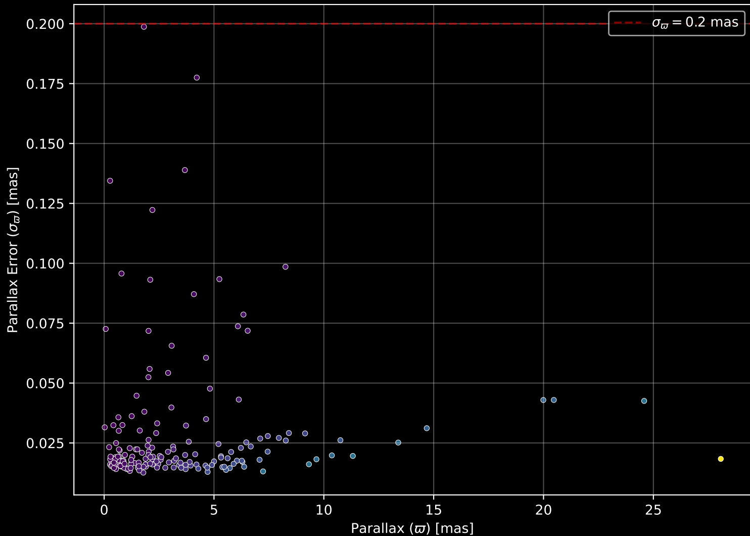
APOGEE DR17 Field: [K2_C4_170-31_btx] Parallax Quality (n= 172)
